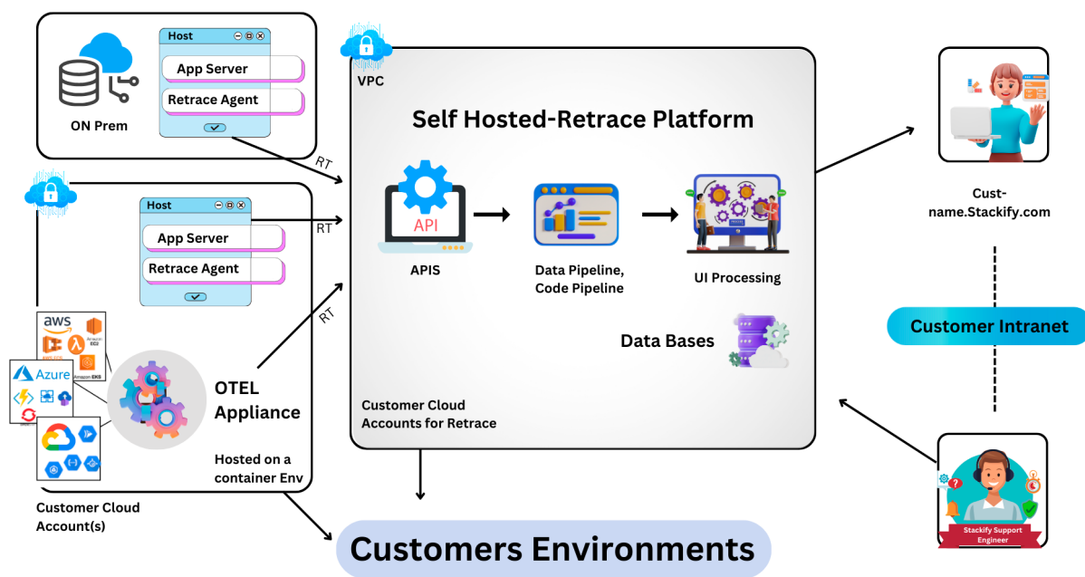
High-level overview of a Self-Hosted Retrace deployment
